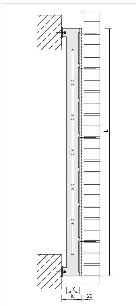
▲ Windpostanker HV-WP
