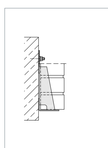
▲ For small loads
