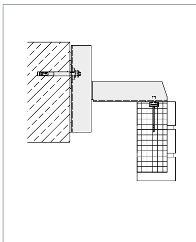
▲ FB-G, central elevation
