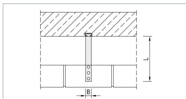
▲ MOSO® wall anchor MA-A
