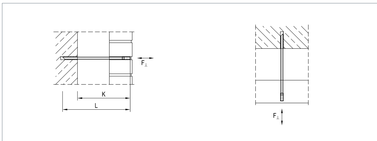
▲ MOSO® scaffold anchor GA-Z
