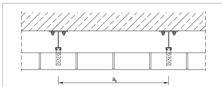
▲ Wind post anchors at variable intervals a_k
