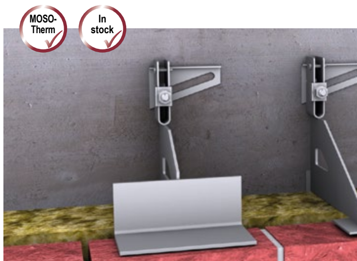
▲ MOSO® single-bracket anchor EK-W as an initial anchor after an expansion joint
