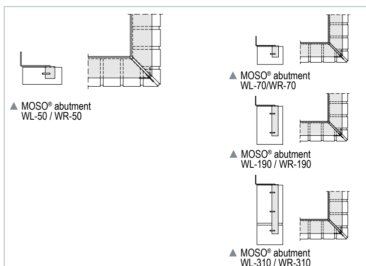
▲ Diverse abutments in corner area, type WL
