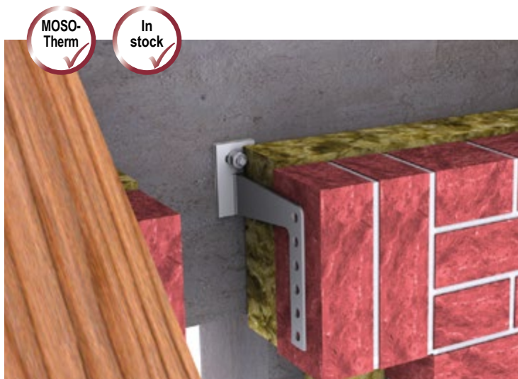
▲ Lintel support with MOSO® single-bracket anchor EK-G
