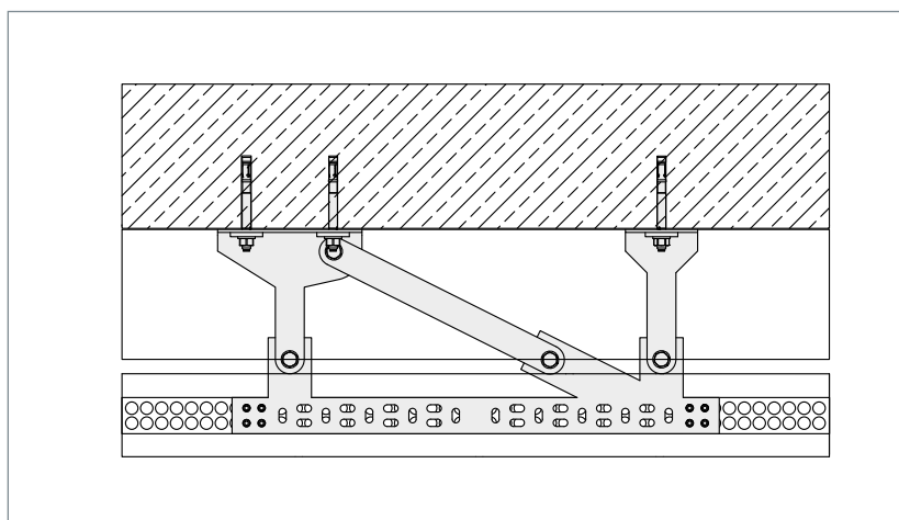
▲ EK-EB for earthquake protection, combined with MOSO® perforated strip
