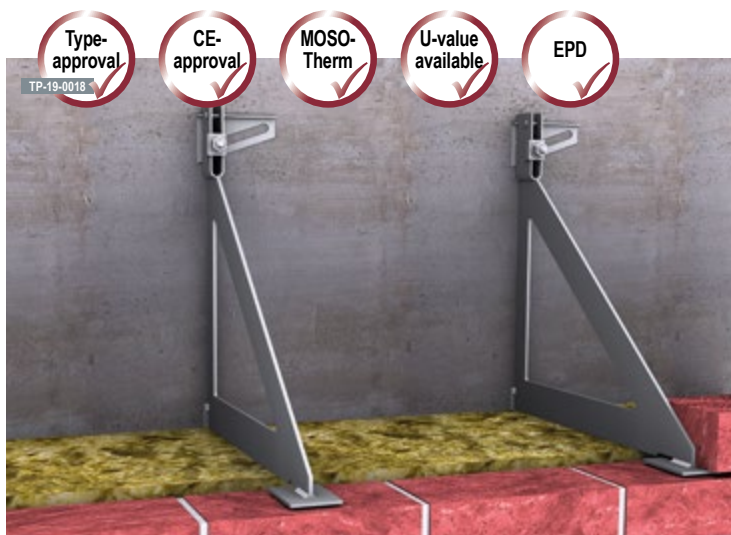
▲ Wall support with MOSO® single-bracket anchor EK-U
