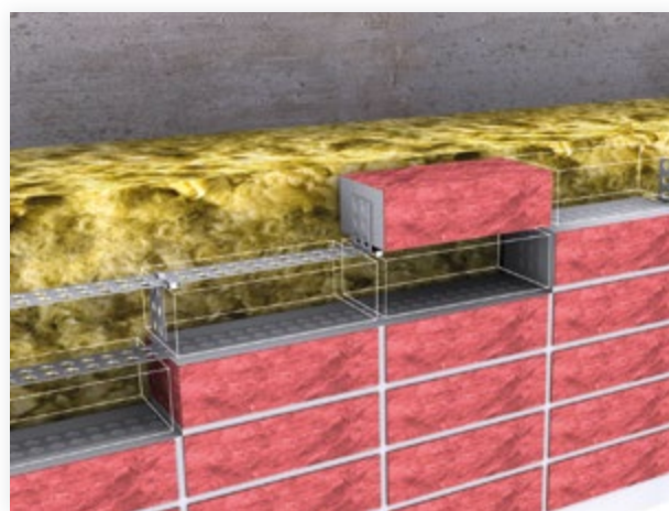
▲ Application for cross joints
