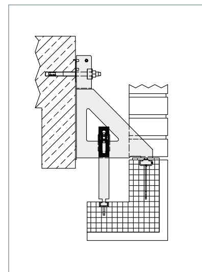
▲ Precast part fixing with anti-tilt device (ZK bracket) on standard FB-U bracket
