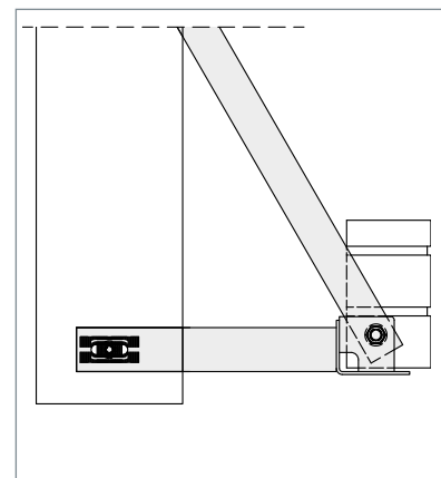
▲ WK-ZS with flat support in alignment with the reinforced concrete structural edge
