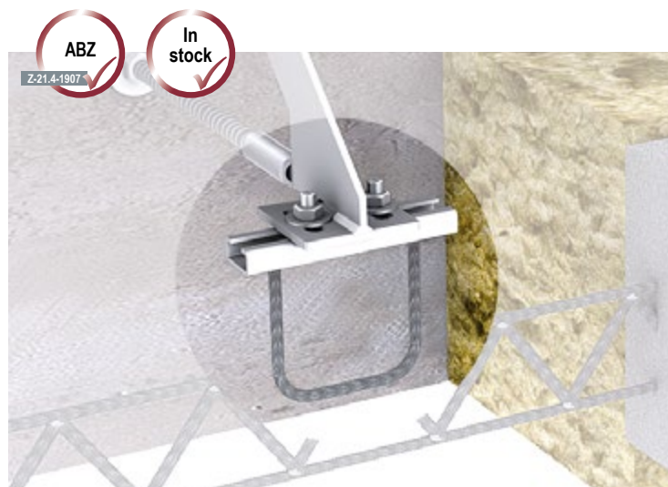
▲ Precast lintel with MOSO® anchor channel MBA-ES set in concrete
