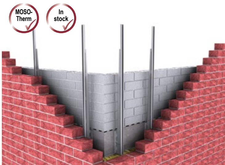
▲ Fascia anchoring with MOSO® horizontal connection HV-A
