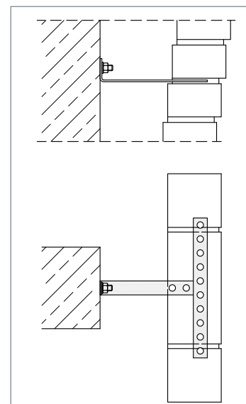
▲ For stepped brickwork
