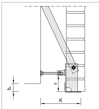
▲ WK-ZV with offset
