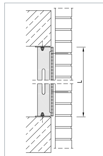
▲ Wind post anchor HV-WPS between reinforced concrete ceilings
