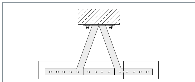
▲ Horizontal securing of a long masonry pier with a narrow reinforced concrete support in the carcass as anchoring base
