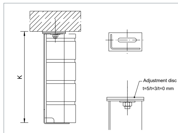
▲ WK-I bracket
