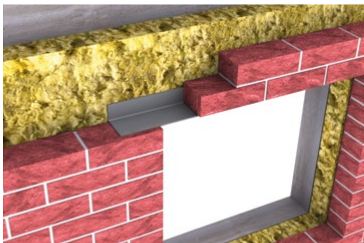
▲ Opening overlap with MOSO® angle bearing WA-Ü
