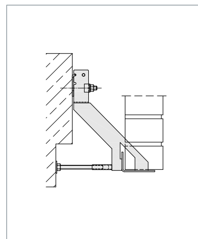
▲ WK-DS with longer pressure screw
