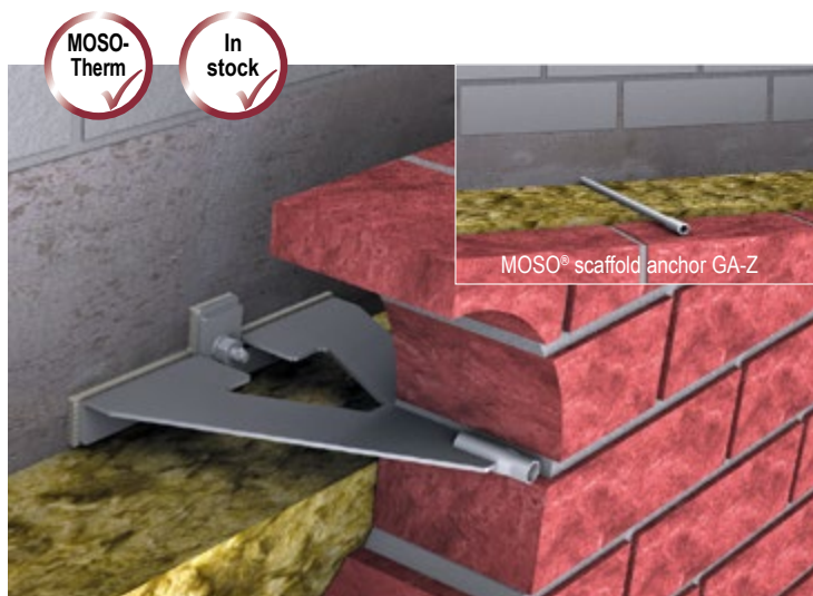
▲ Anchoring with MOSO® scaffold anchor GA-Q, also available with MOSOTherm
