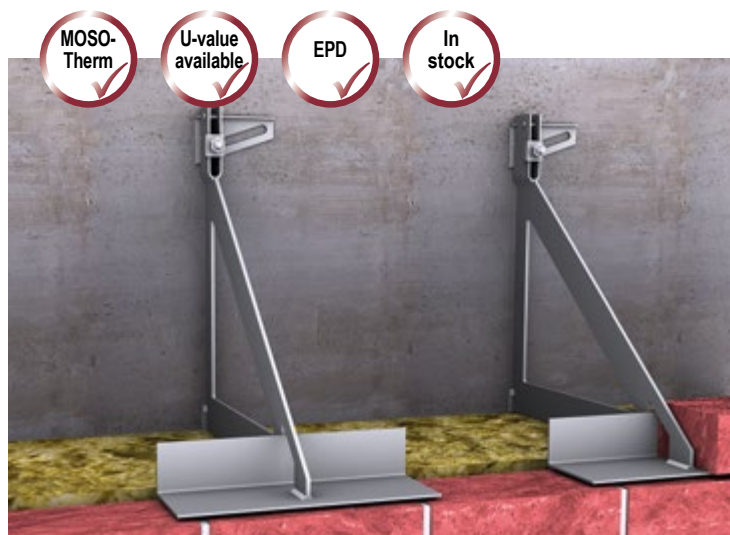
▲ Wall support with MOSO® single-bracket anchor EK-L
