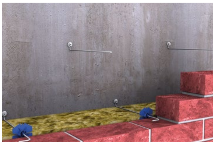
▲ Anchoring with MOSO® horizontal connection HV-L
