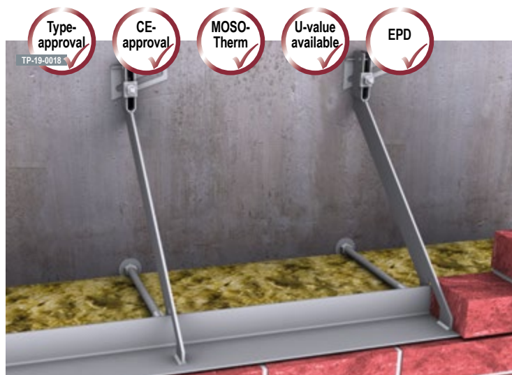
▲ Wall support with MOSO® angle-bracket anchor WK-D
