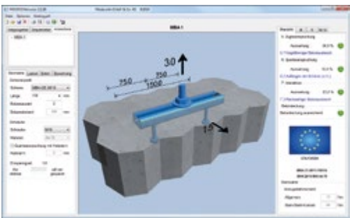
▲ Surface MBA-CE in our free dimensioning software MOSOConstructor
