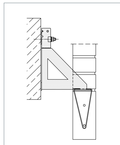
▲ EK-U with wall tie type 2
