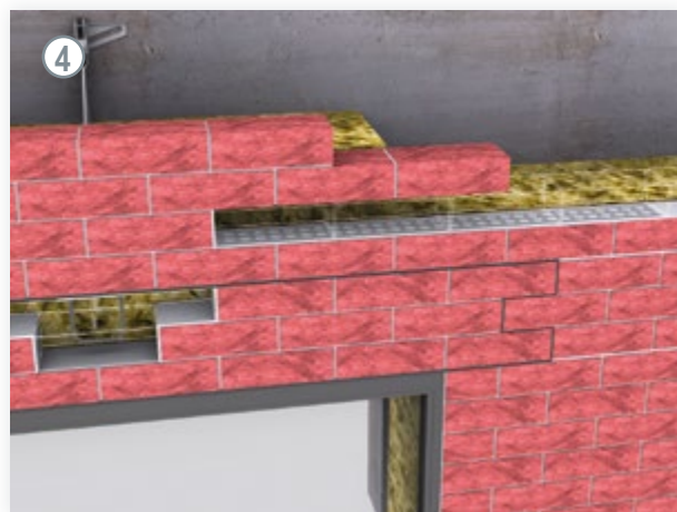
▲ Lintel mounted on one side
