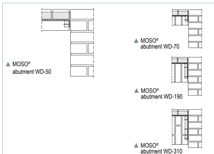
▲ Diverse abutments near expansion joints, type WD
