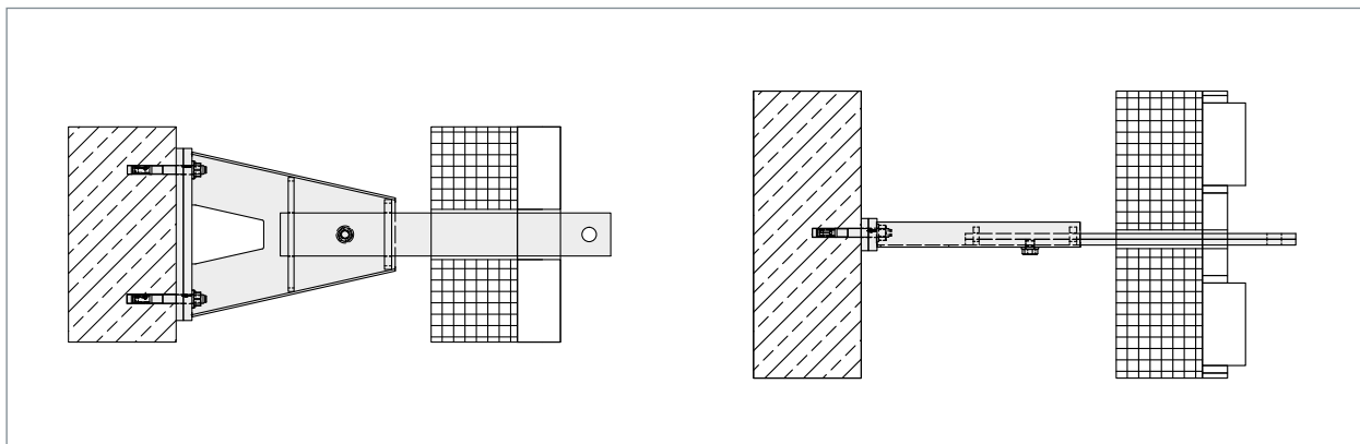
▲ For anchoring in element facades with low horizontal joint thickness
