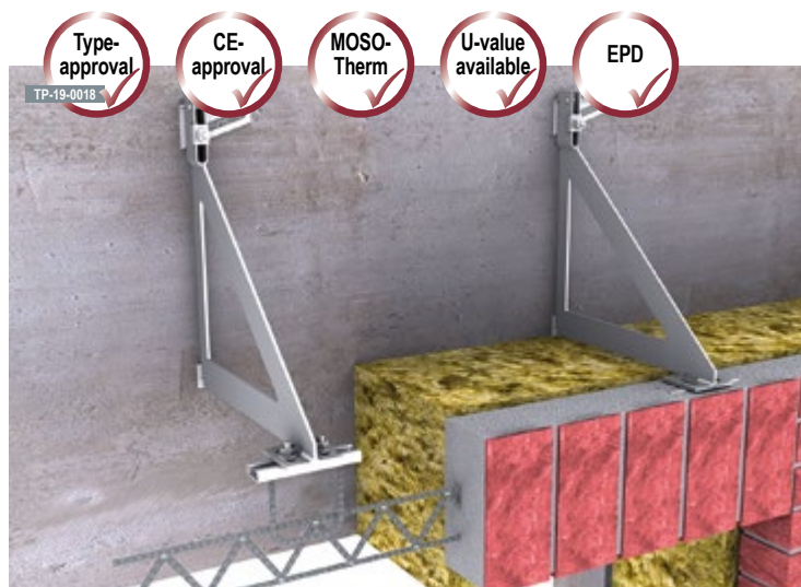
▲ Lintel support with MOSO® fixing for precast parts FB-U
