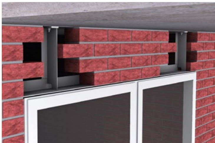
▲ WK-I bracket under balcony slab
