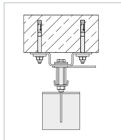
▲ From 20 mm: Hat profile between carcass and bracket
