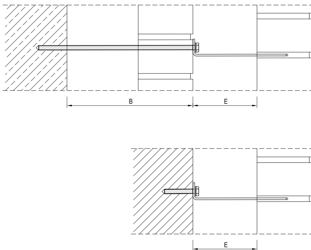
▲ MOSO® horizontal connection HV-L, anchoring in perforated brick possible
