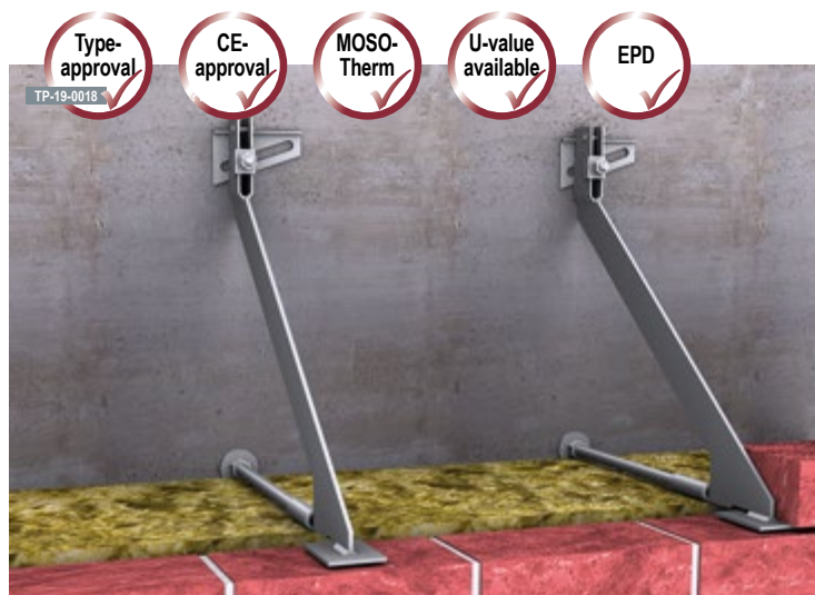
▲ Wall support with MOSO® single-bracket anchor EK-D
