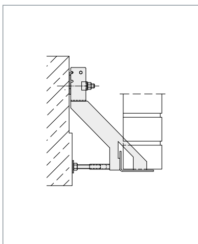
▲ Pressure screw adjustable \pm 15 mm
