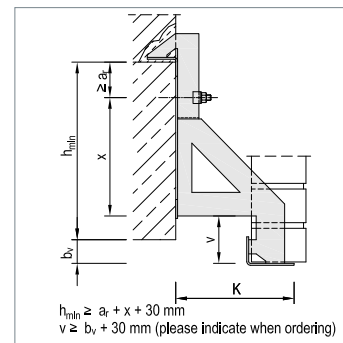
▲ WK-KV with offset
