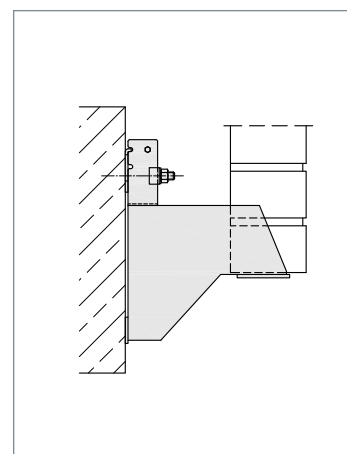
▲ With raised supporting plate
