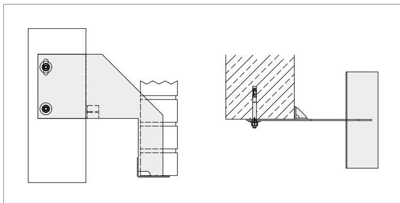
▲ Corner anchor as an alternative to the tie rod
