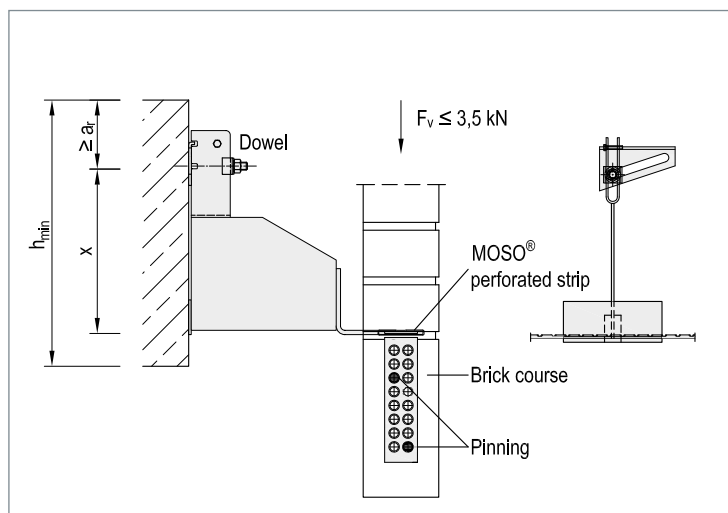
▲ Profile and frontal view of support bracket EK-W with MOSO® perforated strip
