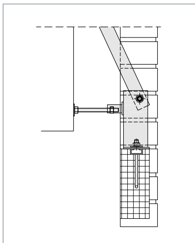
▲ Corner bracket for precast parts FB-ZBV
