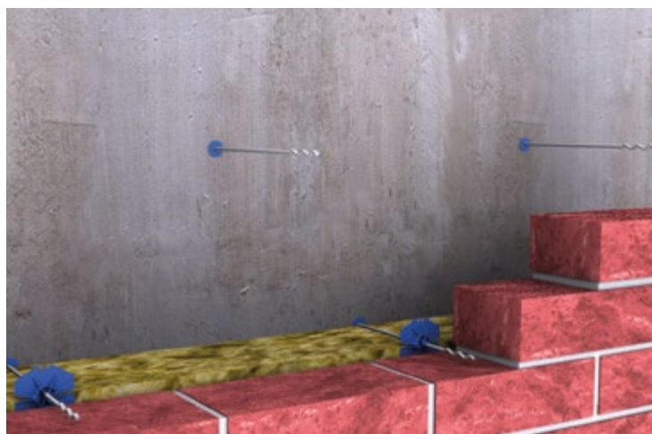
▲ Anchoring with MOSO® horizontal connection HV-DAZ
