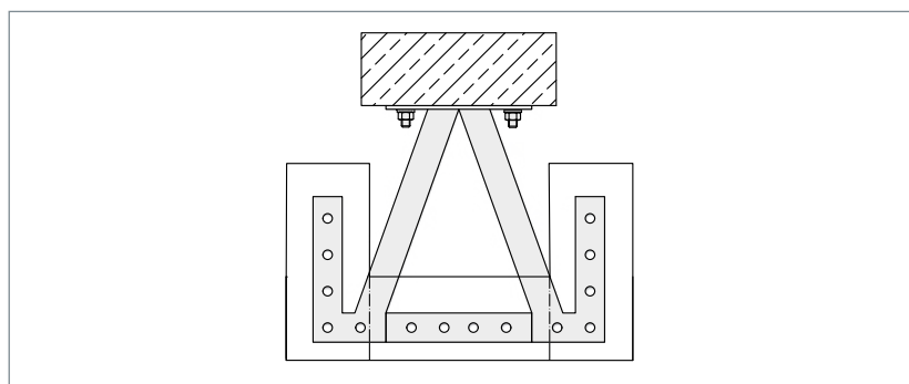
▲ Horizontal securing of a U-shaped masonry pier
