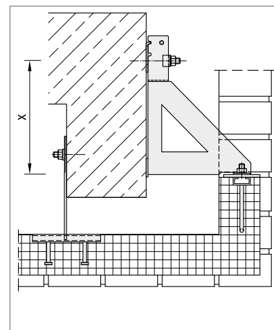
▲ FB-U with FB-ZK as support for the prefabricated ceiling
