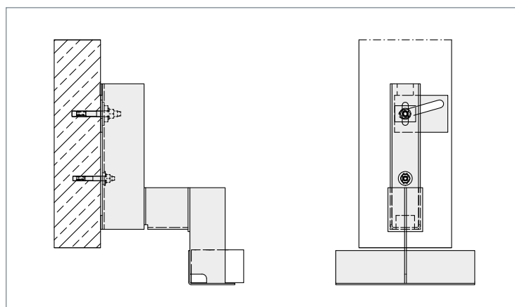
▲ Single anchor mounting on narrow carcass, 2nd anchor as anti-rotation device
