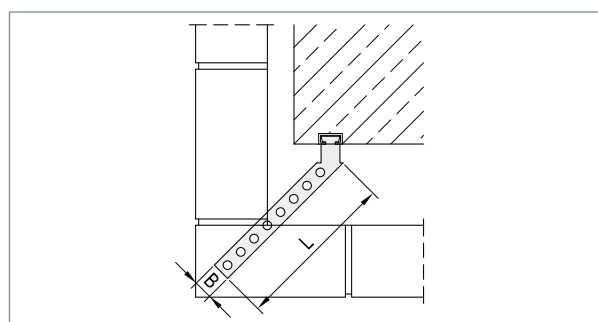
▲ MOSO® wall anchor MA-AW
