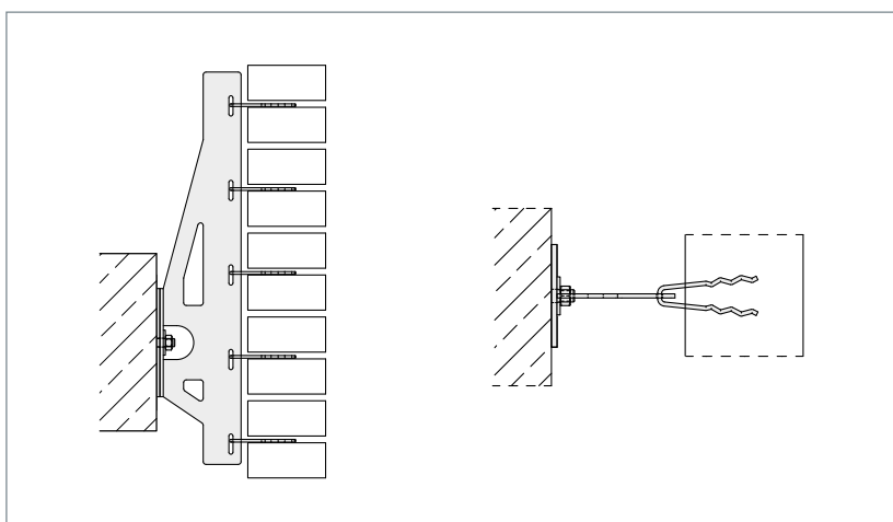
▲ HV-AS Solution without MOS channel
