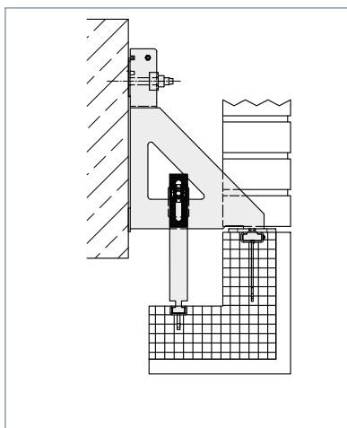
▲ FB-U with FB-ZK as anti-rotation lock of the lintel
