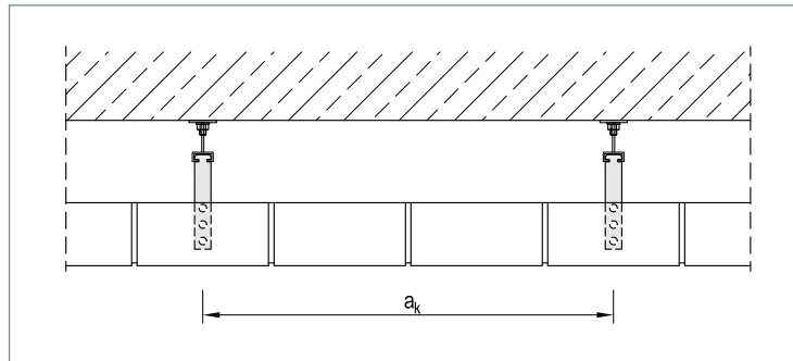
▲ Horizontal connection HV-A
