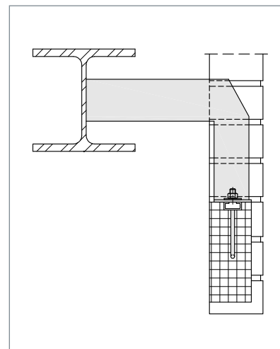
▲ To connect to a steel profile
