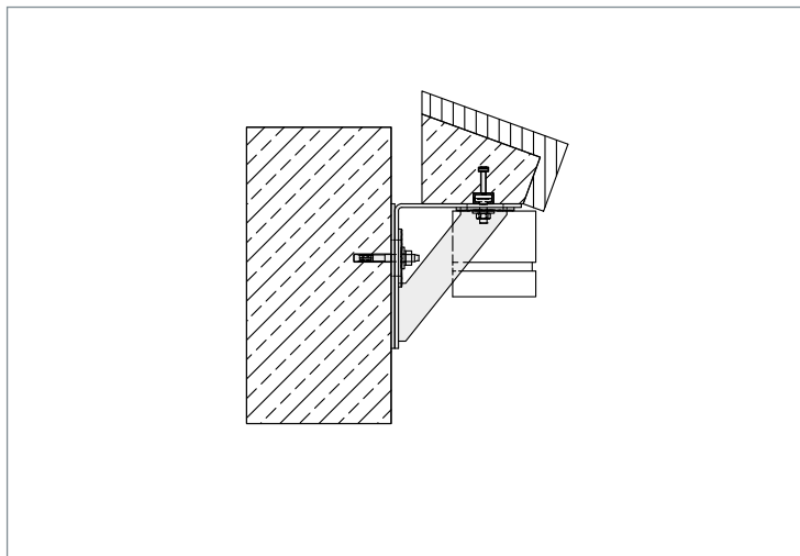
▲ Window sill bracket cantilever with screw connections in CE rail
