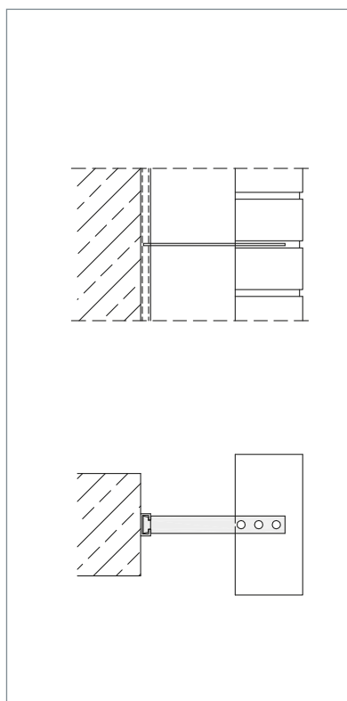
▲ To connect to a channel
