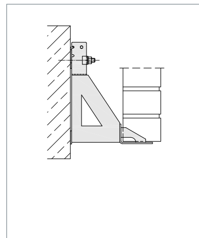
▲ Type WK-NX with welded-in gusset
