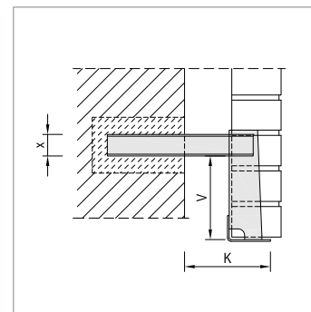
▲ WK-MV with offset
