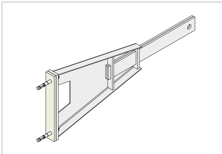
▲ Special permanent scaffolding anchor for large shell spacings
