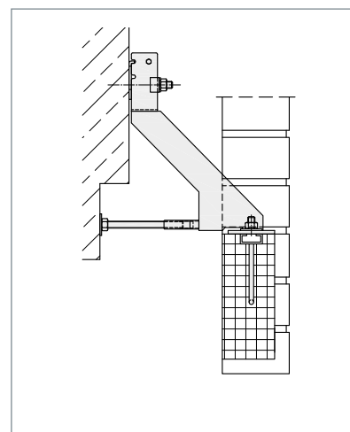
▲ FB-D with long pressing screw
