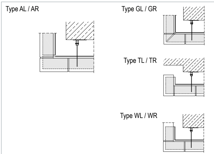
▲ Various corner and edge formations
