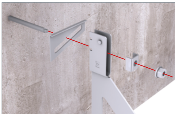
▲ Insert the dowels after approval, place the slotted hole plate and support anchor on the dowel anchor rod.
