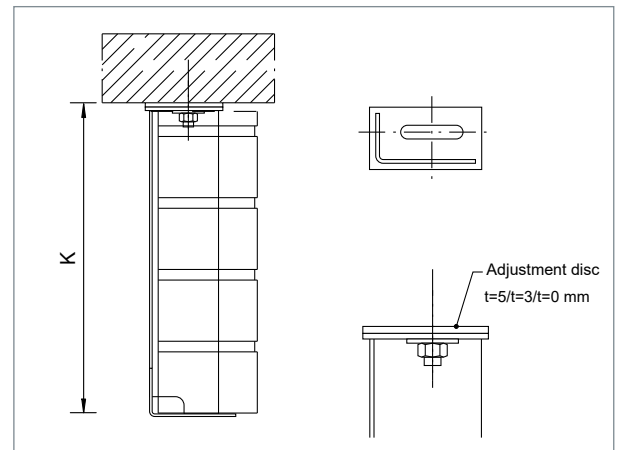
▲ WK-I bracket
