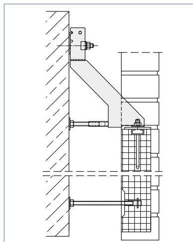
▲ FB-D with additional pressing screw
