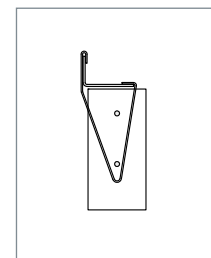
▲ Locally bricked up grenadier layer by means of wire bracket DB-1 below WA-Ü mountable
