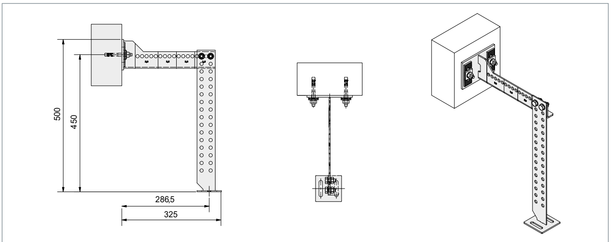
▲ The design of the FB-R allows anchoring, e.g. to reinforced concrete ceilings
