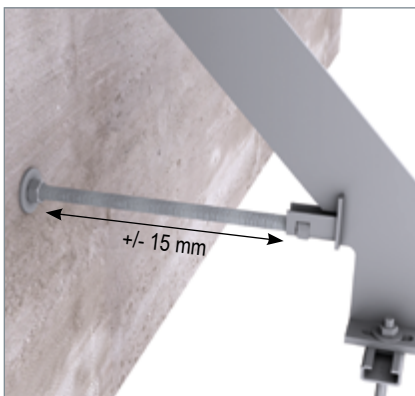
▲ Adjust the pressure screw until it is flush against the shell.
